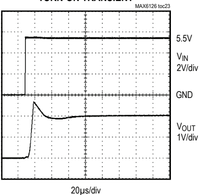
MAX6126_21 TURN-ON TRANSIENT
