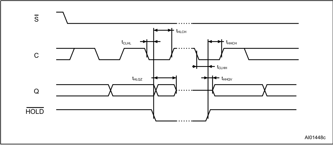
Figure 19. Hold timing
