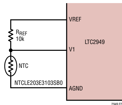
Figure 22. Connecting Thermistors
