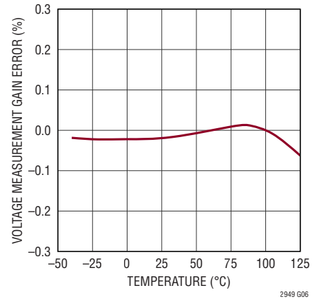
AUXADC Gain Error vs Temperature
