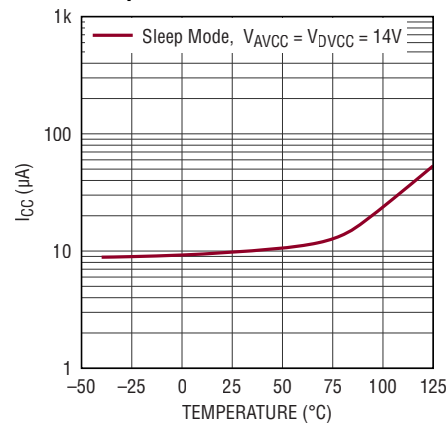
AVCC/DVCC Supply Current Temperature
