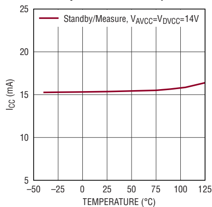
AVCC/DVCC Supply Current Standby/Measure vs Temperature
