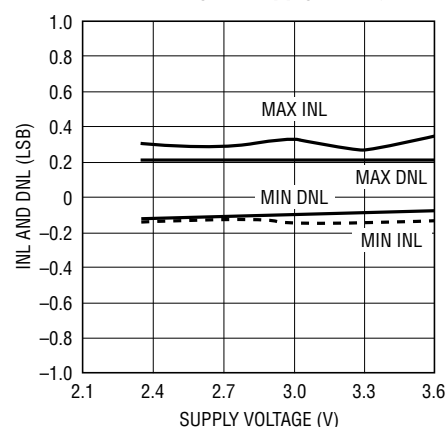
Integral and Differential Nonlinearity vs Supply Voltage
