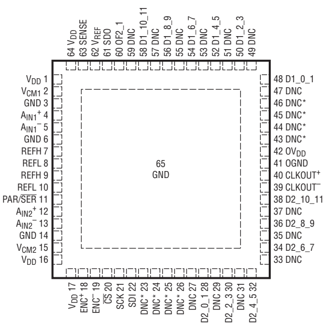
UP PACKAGE
