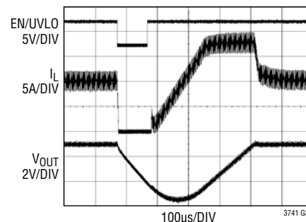
Shutdown and Recovery 1.5nF Soft-Start Capacitor
