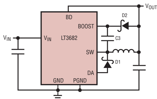
(5b) For 2.5\text{V} < V_{\text{OUT}} < 2.8\text{V} ; V_{\text{IN(MIN)}} = 4.3\text{V}
