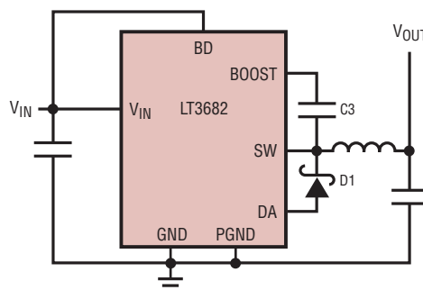
(5c) For V_{\text{OUT}} < 2.5\text{V} ; V_{\text{IN(MAX)}} = 25\text{V}
