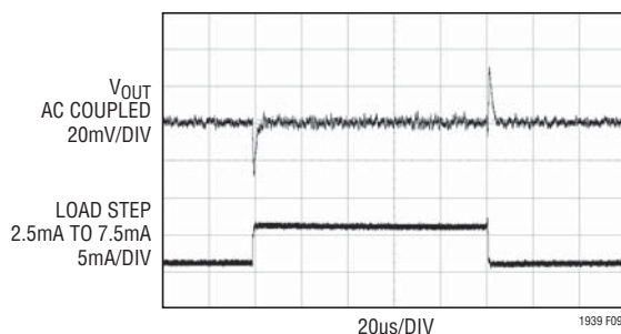
Figure 9. Linear Regulator Transient Response
