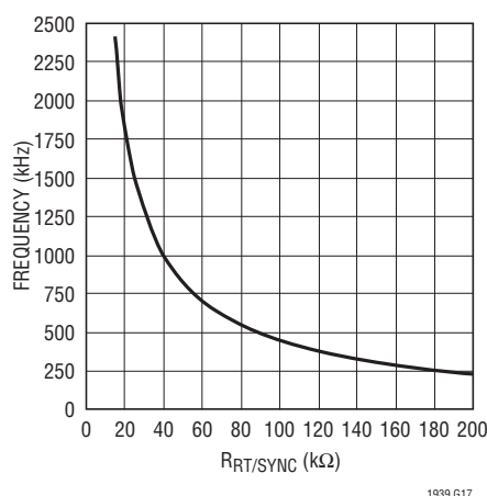
Figure 2. Frequency vs R_T/SYNC Resistance
