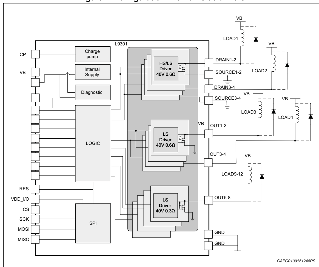
Figure 4. Configuration 1: 8 Low side drivers
