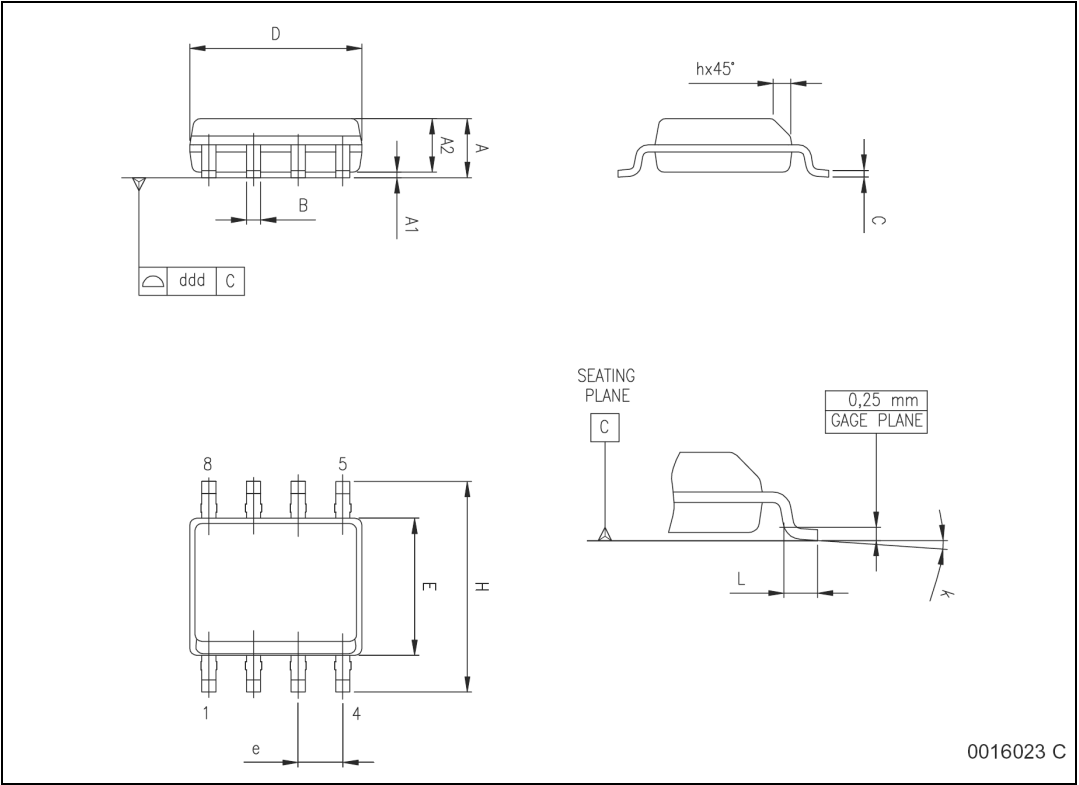
Figure 22. Package dimensions
