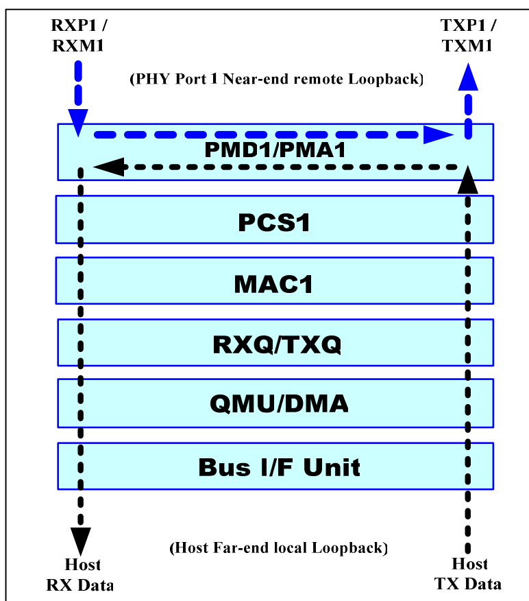
Figure 11. PHY Port 1 Near-end (Remote) and Host Far-end (Local) Loopback Paths
