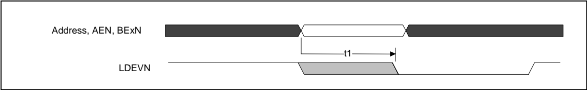
Figure 13. Address Latching Cycle for All Modes
