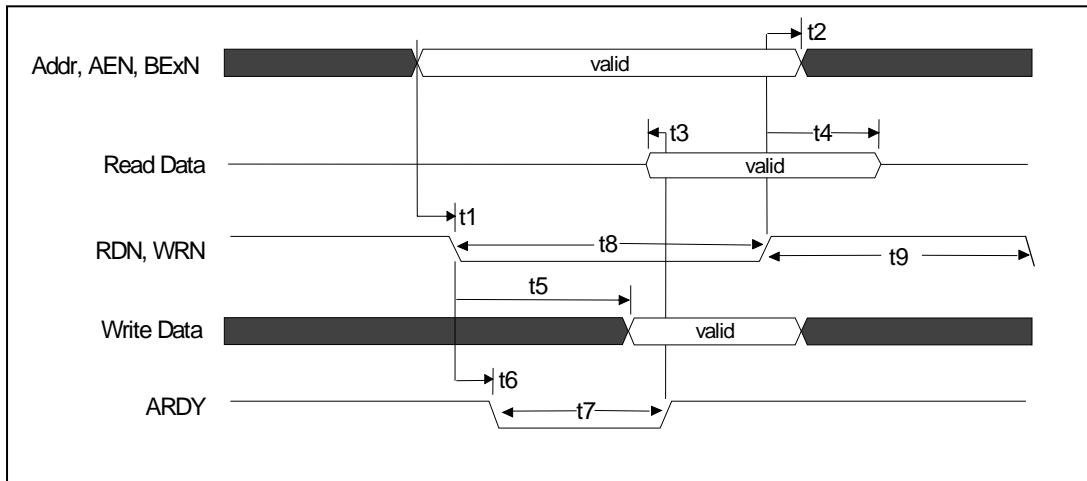
Figure 12. Asynchronous Cycle
