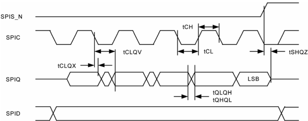
Figure 26. SPI Output Timing
