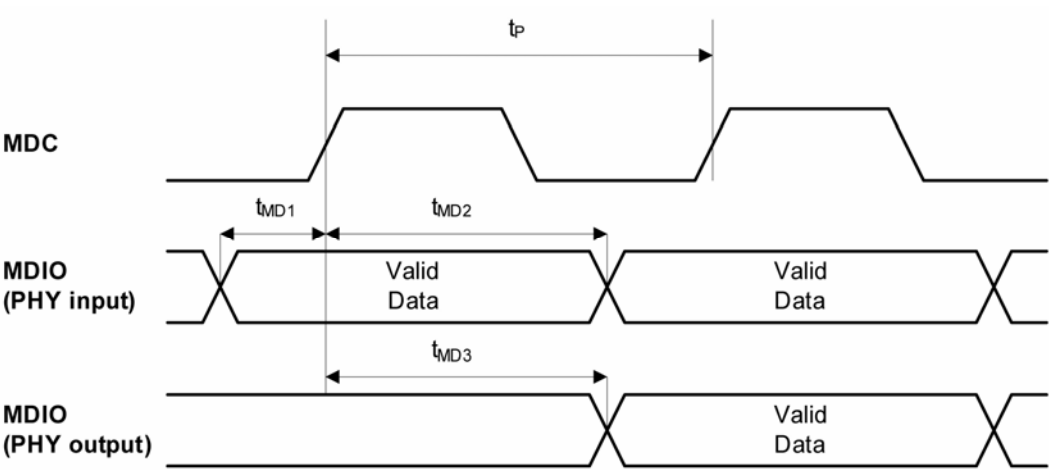
Figure 28. MDC/MDIO Timing
