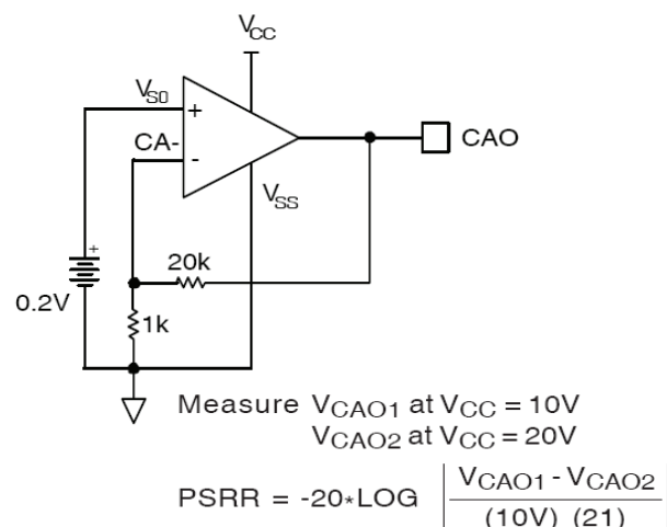
Fig 10. Operational Amplifier Power Supply Rejection Ratio Measurements
