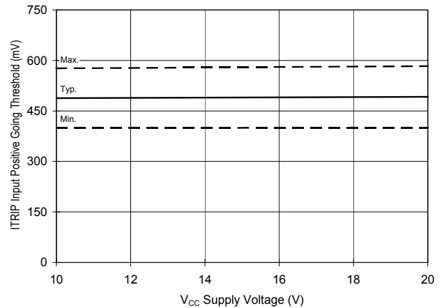
Fig 23b. ITRIP Input Positive Going Threshold
