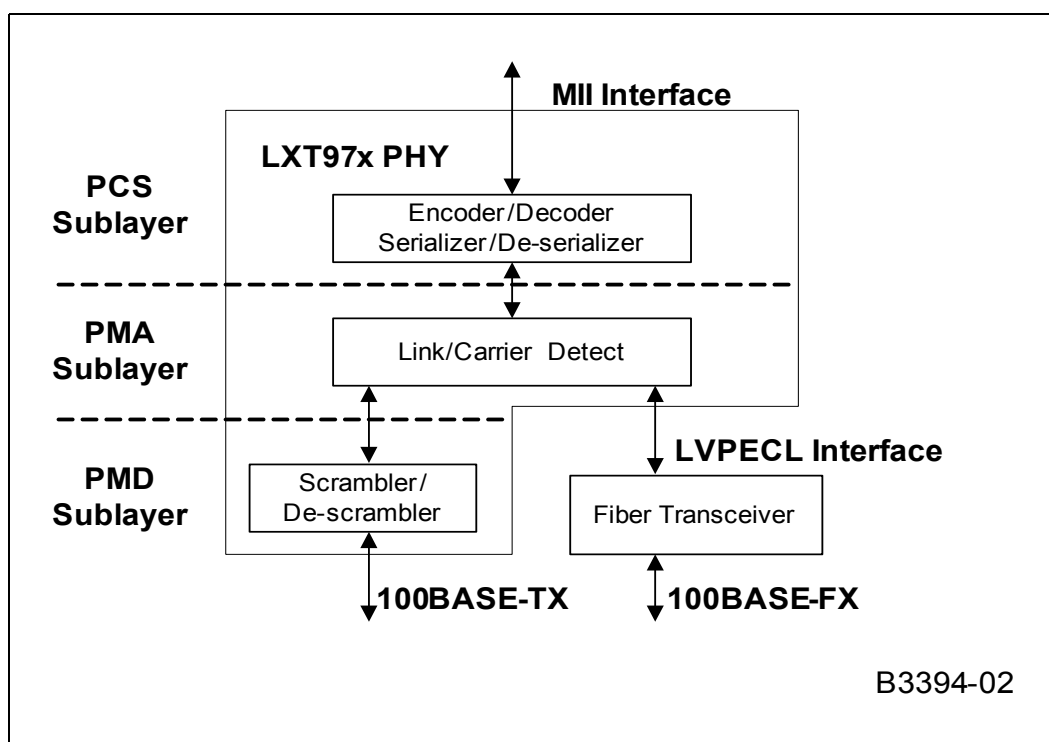
Figure 20 Protocol Sublayers
