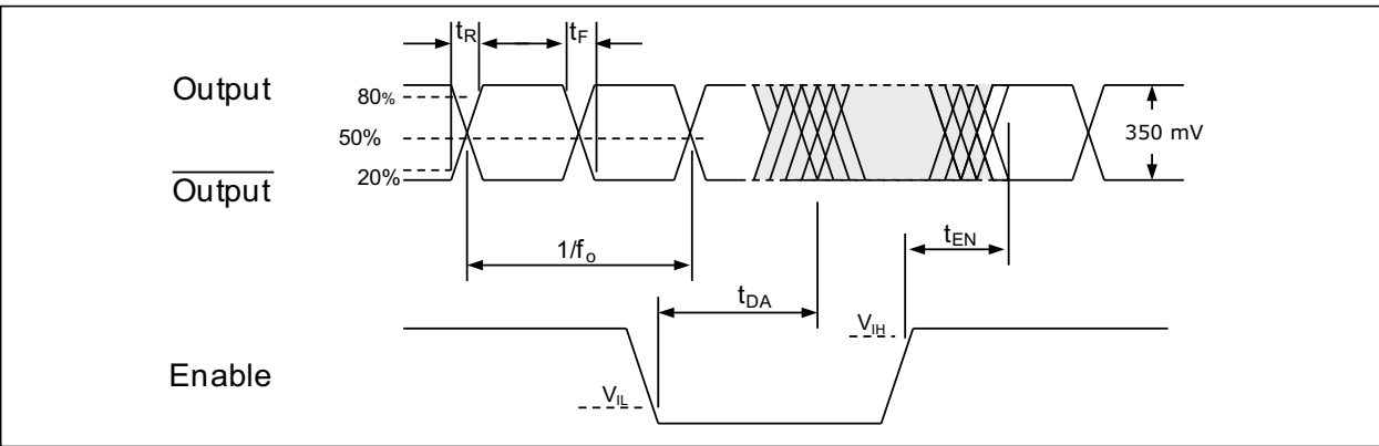
FIGURE 3-3: Output Waveform.
