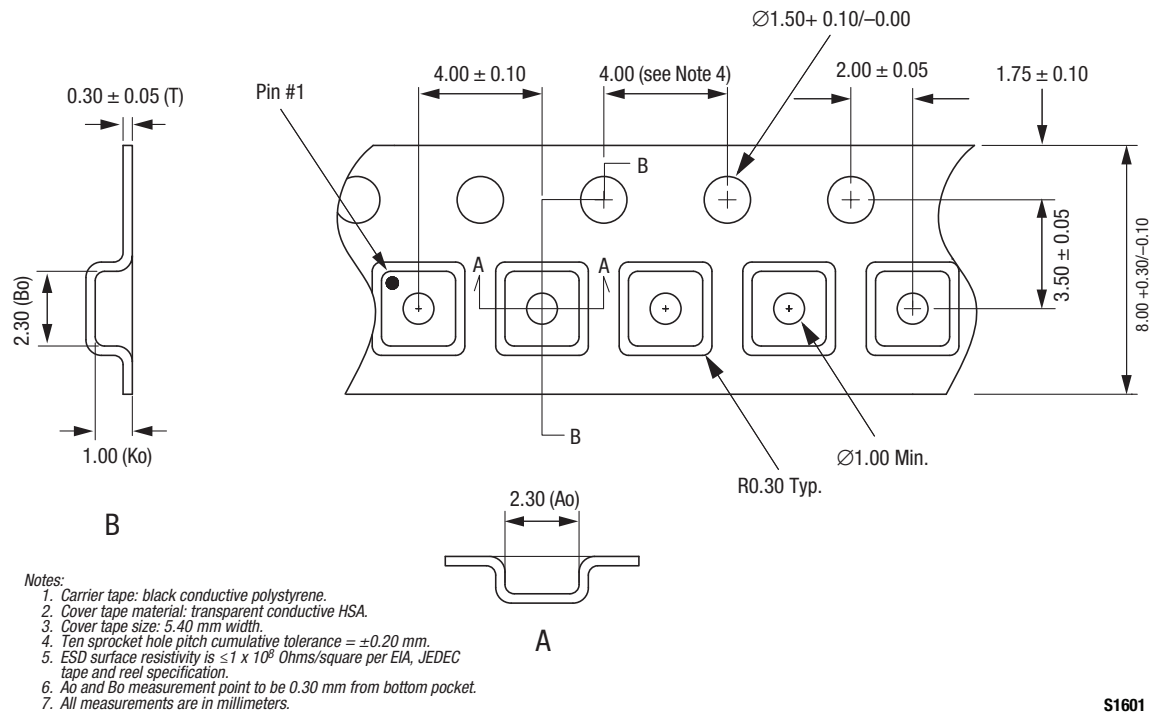
Figure 11. CLA4607-085LF Tape and Reel Dimensions
