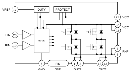
Figure 5. BD6232FP
