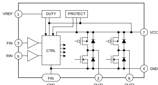
Figure 3. BD6231HFP / BD6232HFP
