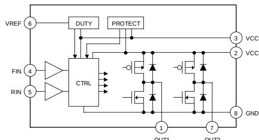
Figure 1. BD6230F / BD6231F
