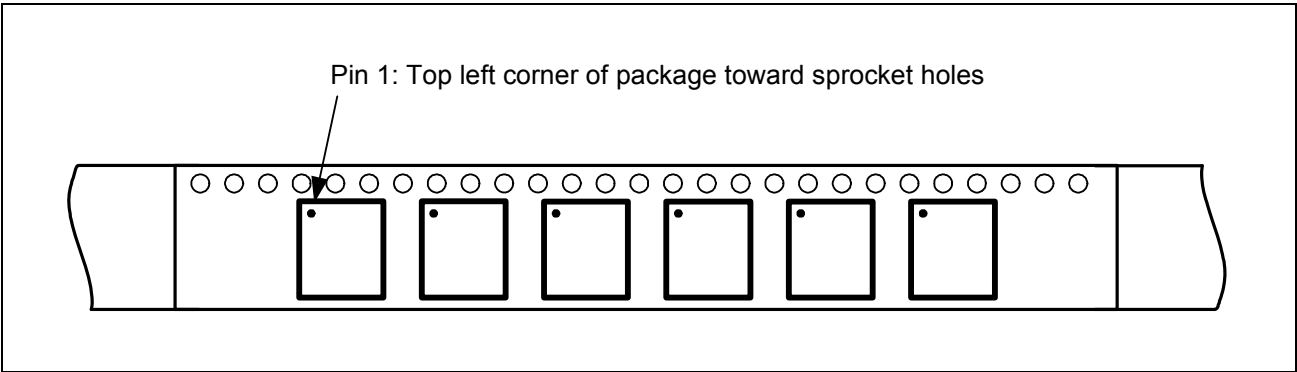
Figure 22: Pin 1 Orientation
