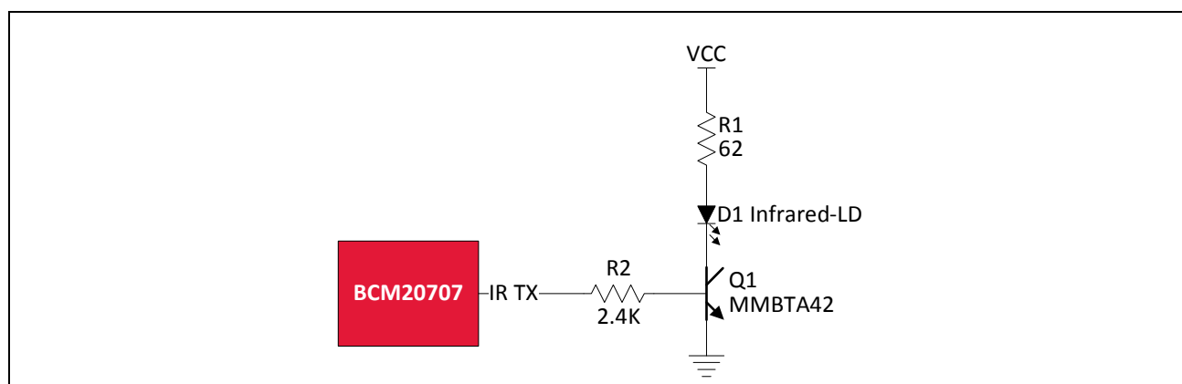
Figure 6: Infrared TX
