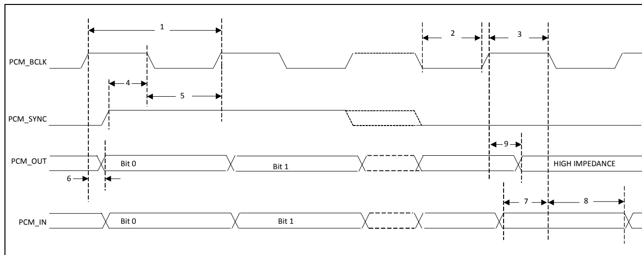
Figure 17: PCM Timing Diagram (Long Frame Sync, Slave Mode)
