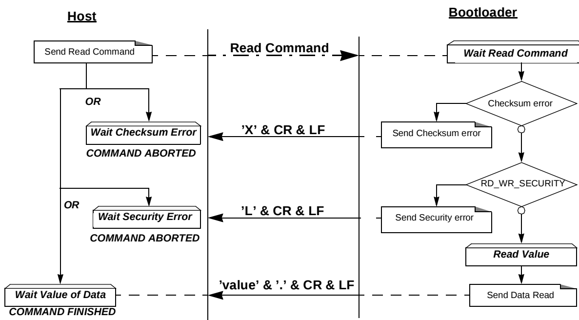
Figure 45. Read Flow
