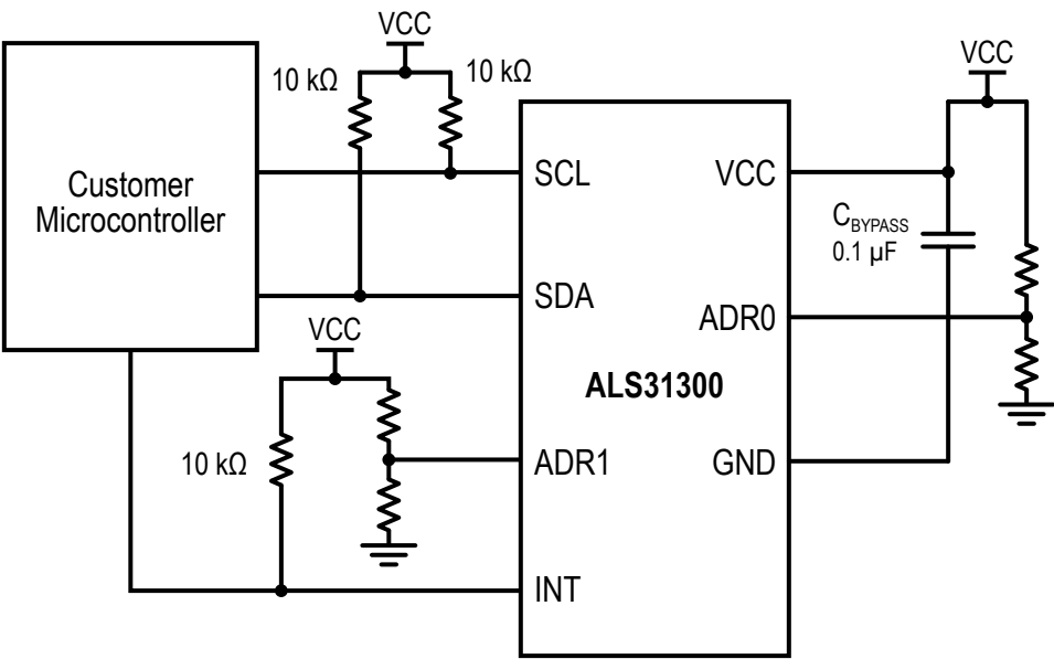
Figure 2: Typical Application
