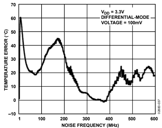
Figure 36. External Temperature Error vs. Differential-Mode Noise Frequency
