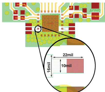
Figure 43. With Impedance Match
