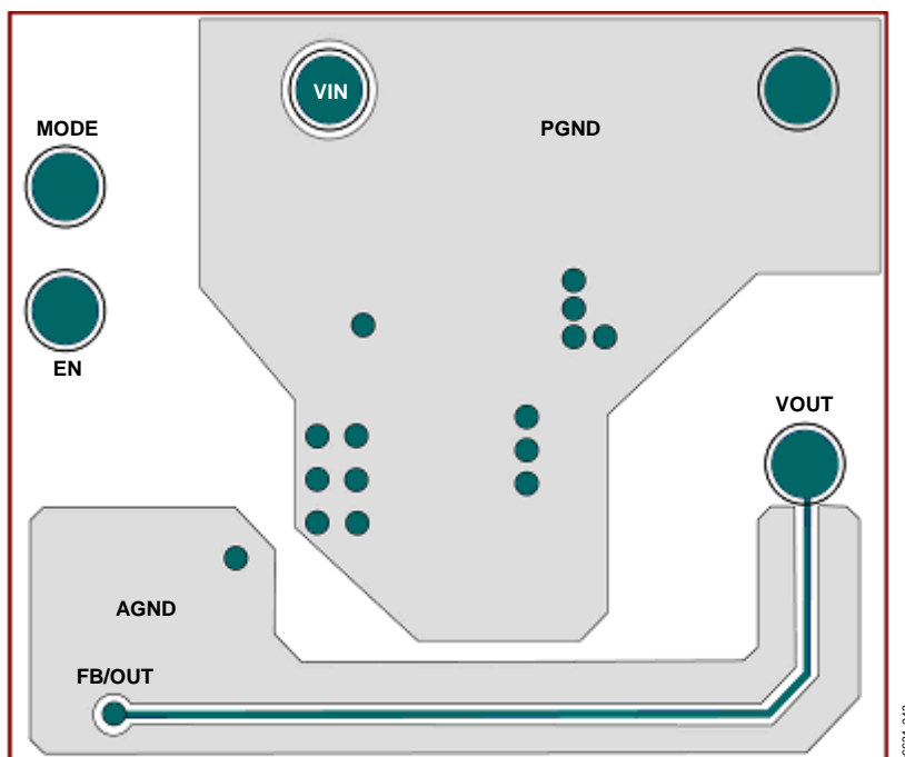
Figure 53. Recommended Layout of the Bottom Layer of the ADP2102 Fixed Output Voltage Options Application Board
