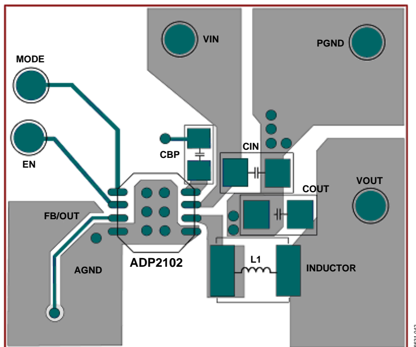
Figure 52. Recommended Layout of the Top Layer of the ADP2102 Fixed Output Voltage Options Application Board
