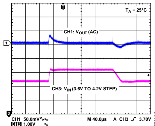
Figure 37. Line Transient Response ( V_{OUT} = 1.8 V)
