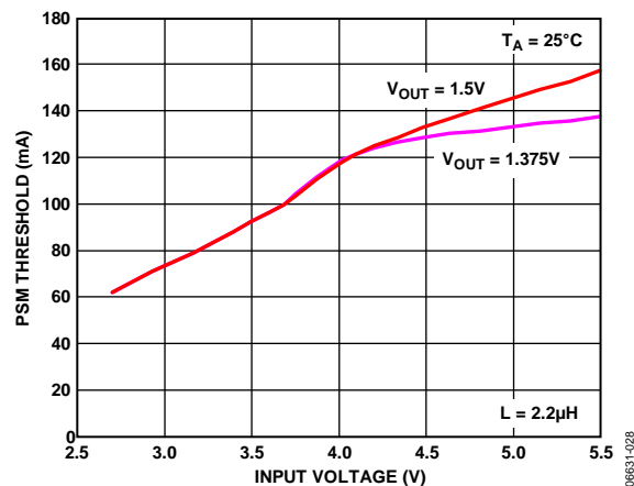
Figure 31. Typical PSM Threshold vs. Input Voltage
