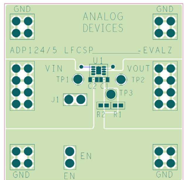
Figure 44. Example ADP124 / ADP125 LFCSP PCB Layout
