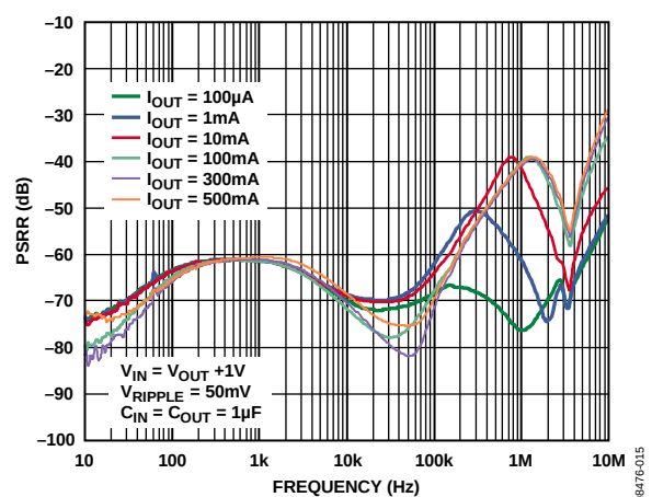
Figure 17. Power Supply Rejection Ratio vs. Frequency, V_{OUT} = 2.8V , V_{IN} = 3.8V
