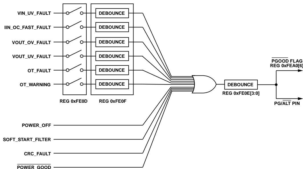
Figure 26. PGOOD Programming
