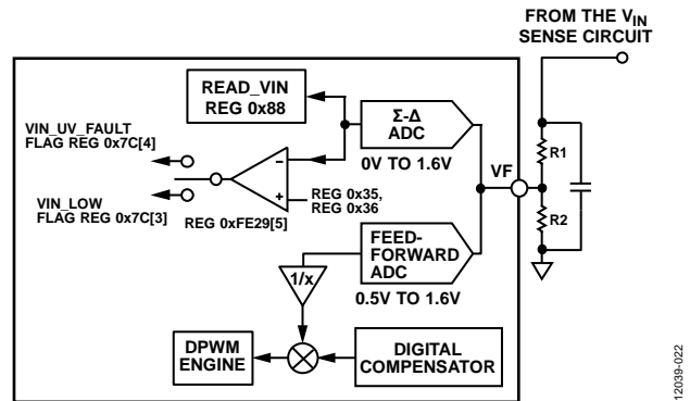
Figure 20. Closed-Loop Input Voltage Feedforward Configuration
