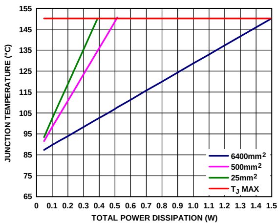
Figure 66. LFCSP, T_A = 85^\circ\text{C}
