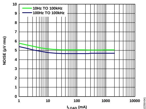
Figure 40. RMS Output Noise vs. Load Current ( I_{LOAD} ), V_{OUT} = 3\text{ V}
