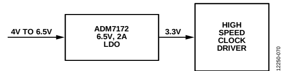
Figure 68. Clock Driver Power
