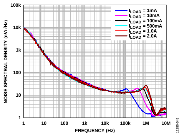
Figure 44. Output Noise Spectral Density, V_{OUT} = 3\text{ V}
