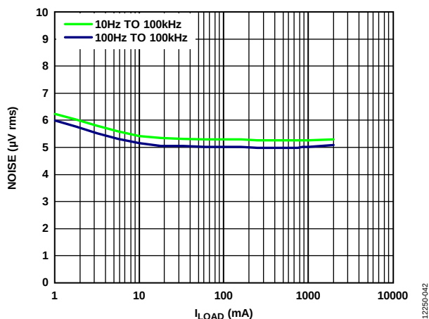
Figure 41. RMS Output Noise vs. Load Current ( I_{LOAD} ), V_{OUT} = 5\text{ V}
