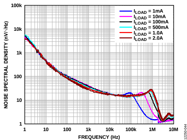
Figure 43. Output Noise Spectral Density, Adjustable Version, V_{OUT} = 1.2\text{ V}
