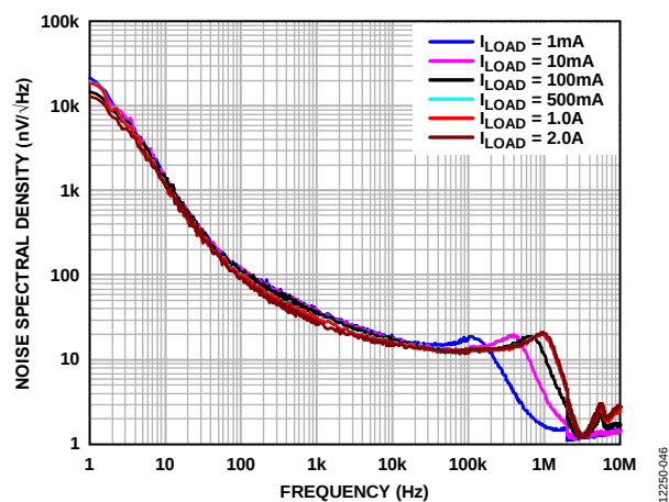
Figure 45. Output Noise Spectral Density, V_{OUT} = 5\text{ V}
