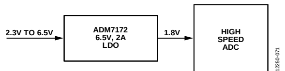
Figure 69. High Speed ADC Power
