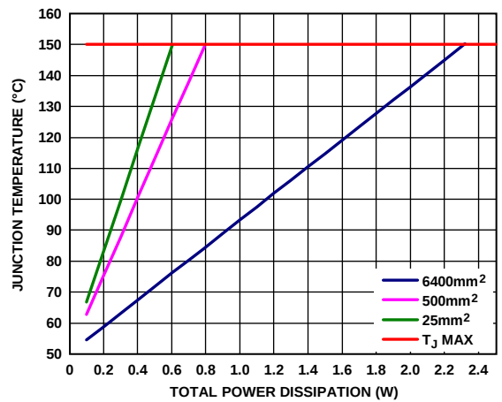
Figure 65. LFCSP, T_A = 50^\circ\text{C}
