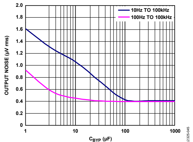
Figure 46. RMS Noise vs. C_{\text{BYP}}
