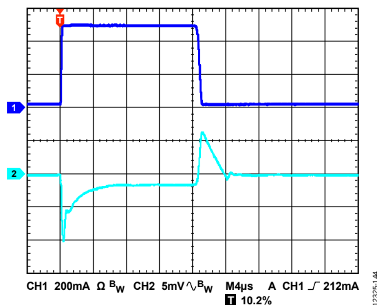
Figure 45. Output Transient Response, V_{\text{OUT}} = 3.3\text{ V} , C_{\text{OUT}} = 10\text{ }\mu\text{F} , CH1 = Load Current, CH2 = V_{\text{OUT}}
