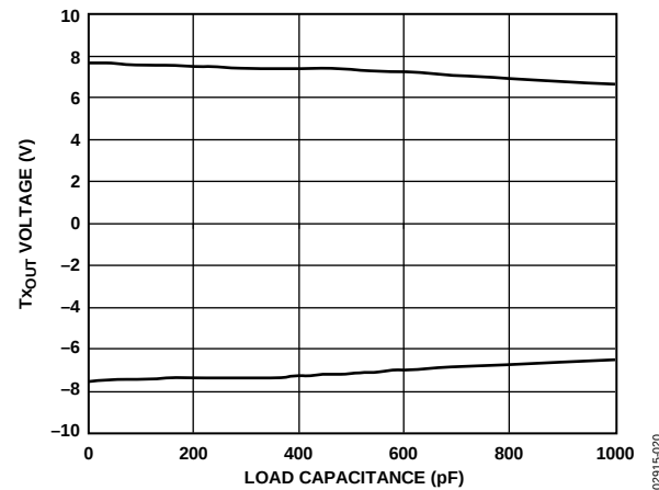
Figure 20. Transmitter Output Voltage High/Low vs. Load Capacitance ( V_{CC} = 3.3 \text{ V} , CLK = 1 Mb/s, R_L = 5 \text{ k}\Omega , ADM3307E)
