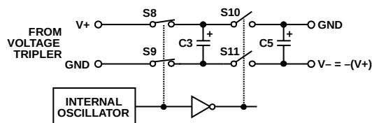
Figure 25. Charge Pump Voltage Inverter
