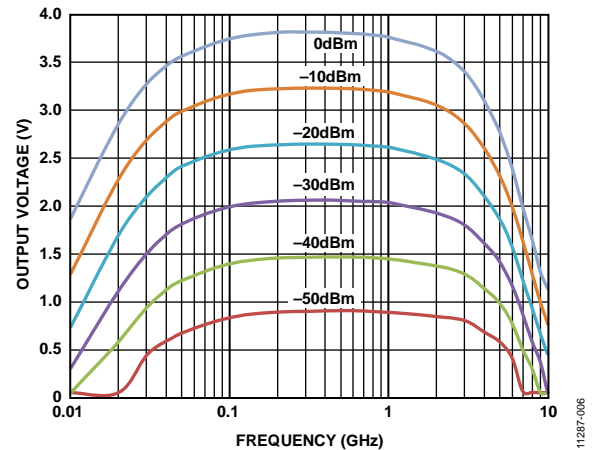
Figure 6. Typical V_{RMS} vs. Frequency for Six RF Input Levels
