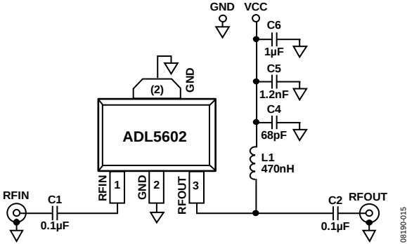
Figure 16. Basic Connections
