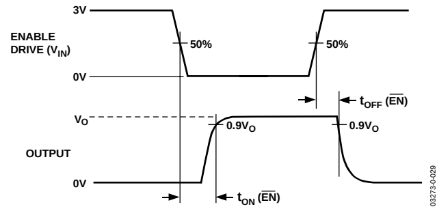
Figure 27. Enable Delay, t_{ON}(\overline{EN}) , t_{OFF}(\overline{EN})
