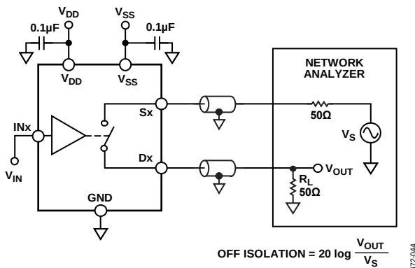
Figure 35. Off Isolation
