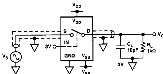
TEST CIRCUIT 5
