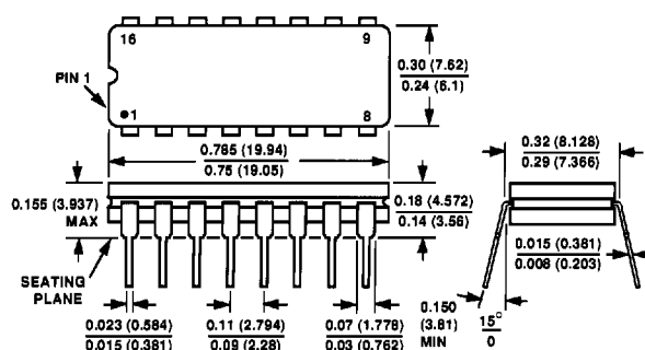
LEAD NO. 1 IDENTIFIED BY DOT OR NOTCH LEADS ARE SOLDER OR TIN-PLATED KOVAR OR ALLOY 42
