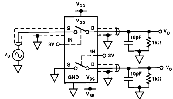
TEST CIRCUIT 6
