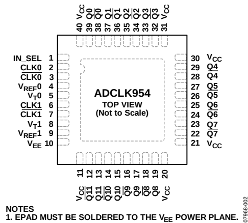
Figure 2. Pin Configuration
