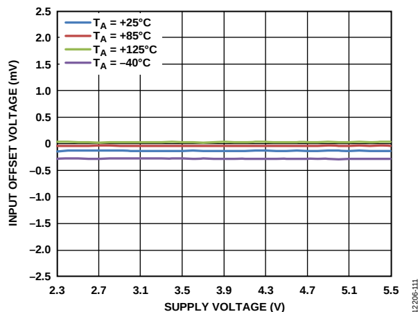
Figure 11. Input Offset Voltage ( V_{OS} ) vs. Supply Voltage ( V_{CC} ), V_{CM} = 1 V for Various Temperatures
