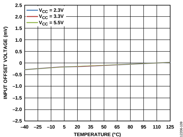
Figure 9. Input Offset Voltage ( V_{OS} ) vs. Temperature for Various Supply Voltages ( V_{CC} ), V_{CM} = 1 V
