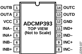
Figure 7. ADCMP393 TSSOP Pin Configuration
