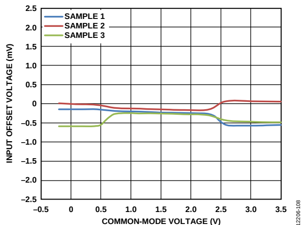
Figure 8. Input Offset Voltage ( V_{OS} ) vs. Common-Mode Voltage ( V_{CM} ), V_{CC} = 3.3 V
