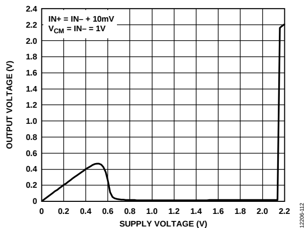
Figure 12. Output Voltage ( V_{OUT} ) vs. Supply Voltage ( V_{CC} ), R_{PULLUP} = 10 k \Omega
