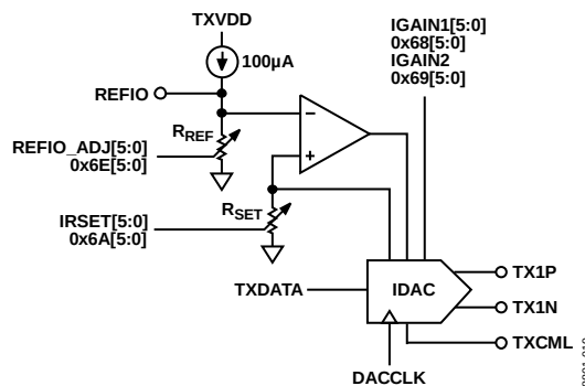
Figure 53. Simplified Block Diagram of I DAC Core
