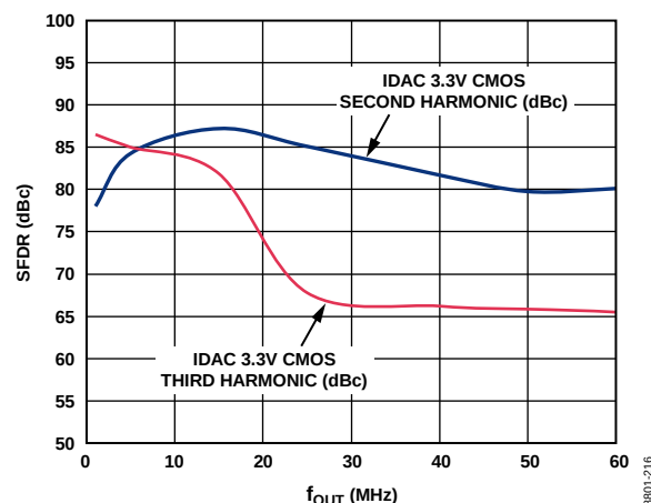
Figure 19. AD9961, Second and Third Harmonic Distortion vs. f_{OUT} , f_{DAC} = 125 MHz, 1×, Digital Scale = 0 dBFS, TXVDD = 3.3 V
