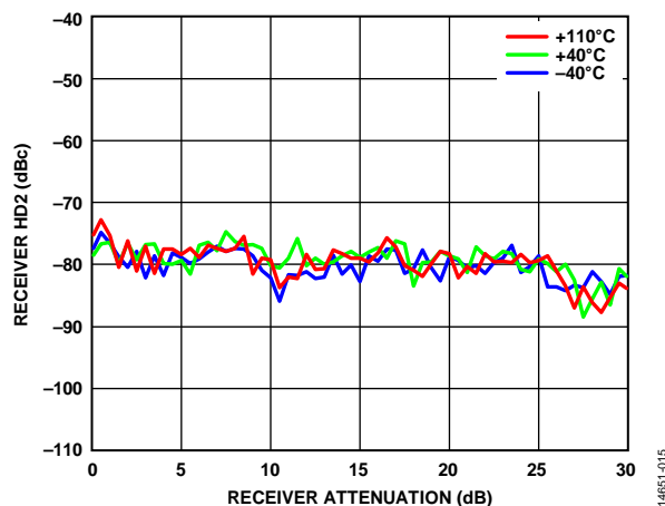
Figure 74. Receiver HD2 vs. Receiver Attenuation, 2600 MHz LO, CW Signal 5 MHz Offset, -20 dBm at 0 dB Attenuation, Input Power Increasing Decibel for Decibel with Attenuation, 40 MHz RF Bandwidth, 122.88 MSPS Sample Rate
