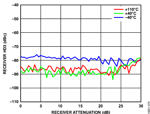
Figure 134. Receiver HD3 vs. Receiver Attenuation, 3500 MHz LO, CW Signal 17 MHz Offset, -14 dBm at 0 dB Attenuation, Input Power Increasing Decibel with Attenuation, 100 MHz RF Bandwidth, 153.6 MSPS Sample Rate
