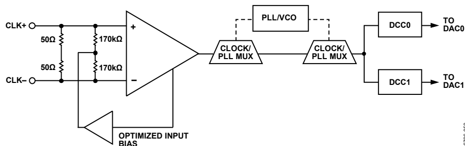
Figure 89. Clock Receiver Input Simplified Equivalent Circuit
