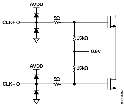
Figure 33. Equivalent Clock Input Circuit
