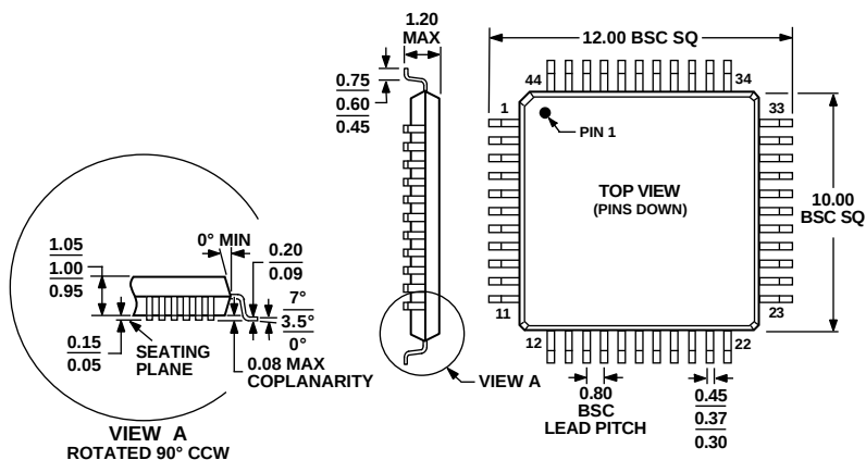
Figure 37. 44-Lead Thin Plastic Quad Flat Package [TQFP]
