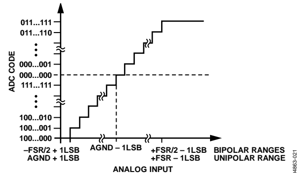
Figure 27. Twos Complement Transfer Characteristic (Bipolar Ranges)
