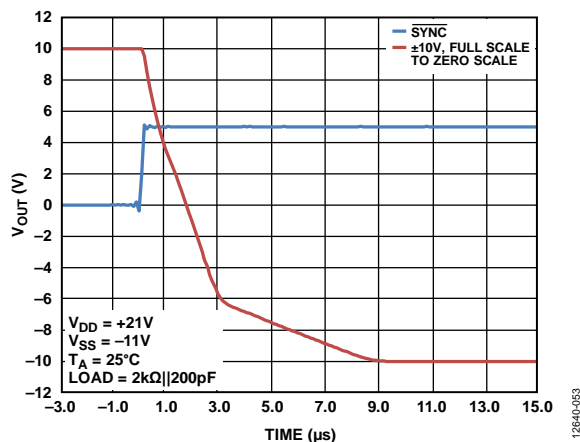
Figure 42. Full-Scale Settling Time (Falling Voltage Step), \pm 10 V Range
