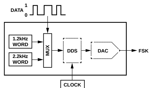
Figure 20. DDS-Based FSK Encoder
