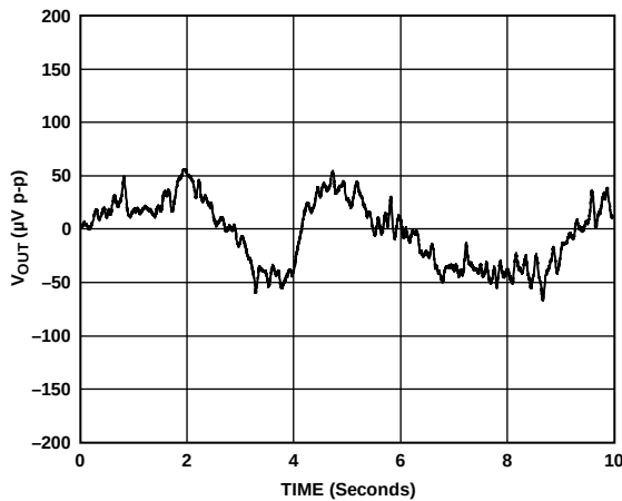
Figure 29. DAC 1/f Noise with External Reference
