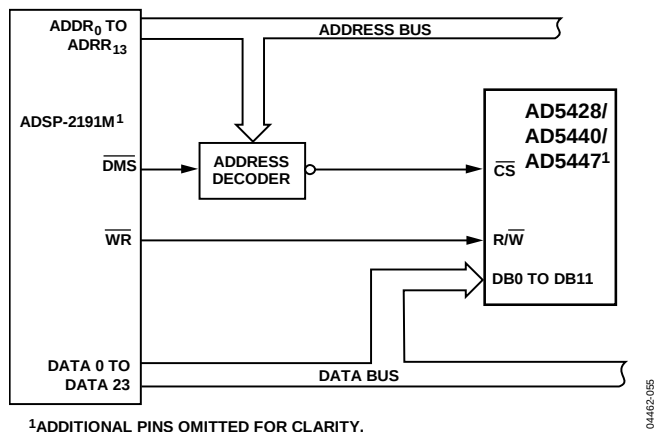
Figure 43. ADSP-2191M-to-AD5428/AD5440/AD5447 Interface
