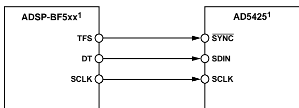
Figure 40. ADSP-BF504 to ADSP-BF592 Device Family to AD5425 Interface (ADSP-BFxx Denotes the ADSP-BF504 to ADSP-BF592)
