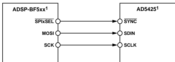
Figure 39. ADSP-BF504 to ADSP-BF592 Device Family to AD5425 Interface (ADSP-BFxx Denotes the ADSP-BF504 to ADSP-BF592)
