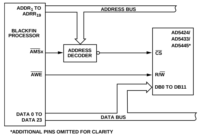
Figure 57. Blackfin Processor-to-AD5424/AD5433/AD5445 Interface
