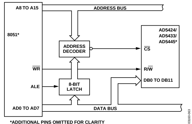
Figure 56. 8xC51-to-AD5424/AD5433/AD5445 Interface
