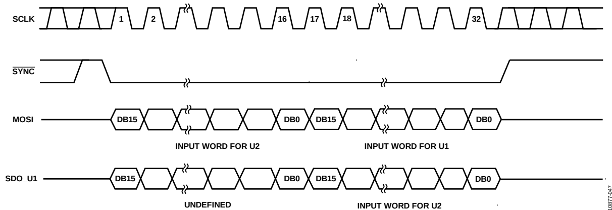
Figure 45. Daisy-Chain Diagram
