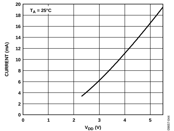
Figure 30. Maximum \overline{A\overline{V}E} Output Current vs. Voltage
