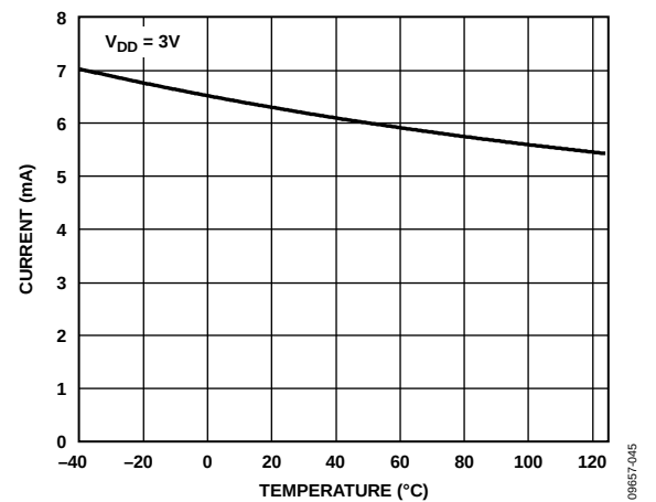
Figure 31. Maximum \overline{A\overline{V}E} Output Current vs. Temperature
