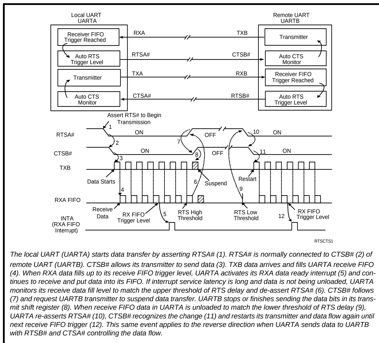
FIGURE 17. AUTO RTS AND CTS FLOW CONTROL OPERATION
