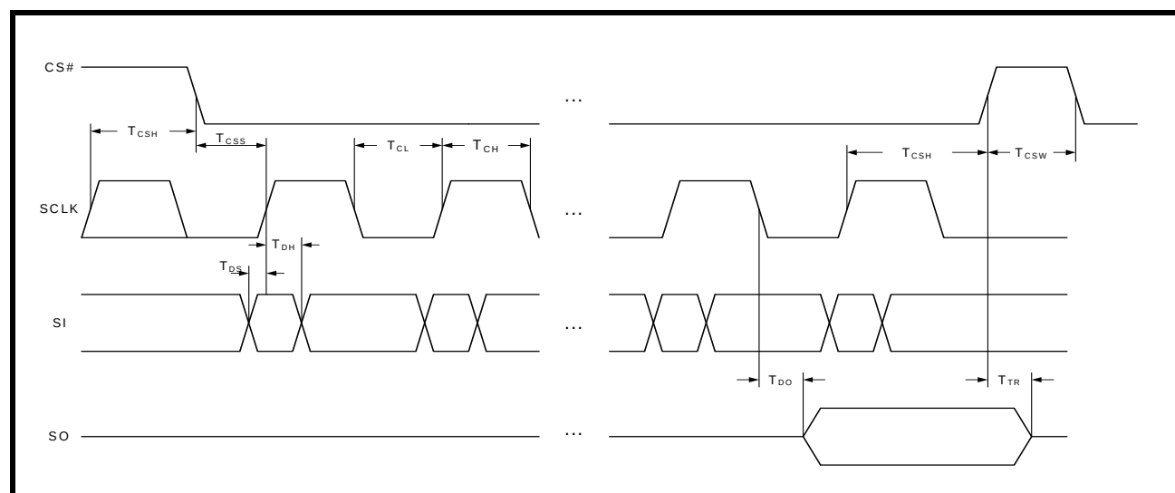
FIGURE 29. SPI-BUS TIMING
