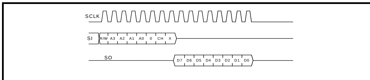
FIGURE 8. SPI READ
