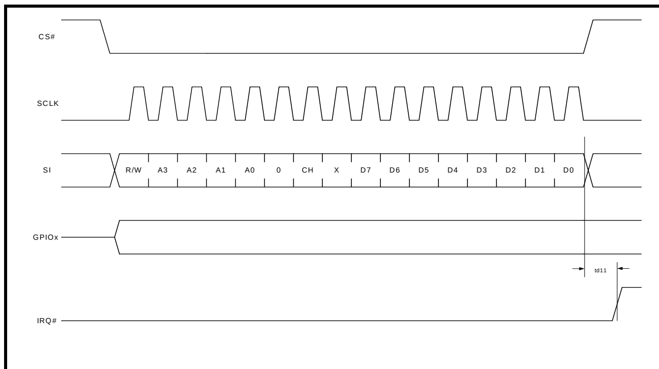
FIGURE 32. SPI WRITE THR TO CLEAR TX INT
