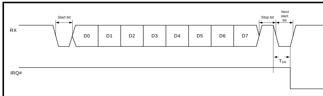
FIGURE 26. RECEIVE INTERRUPT
