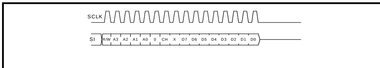
FIGURE 7. SPI WRITE
